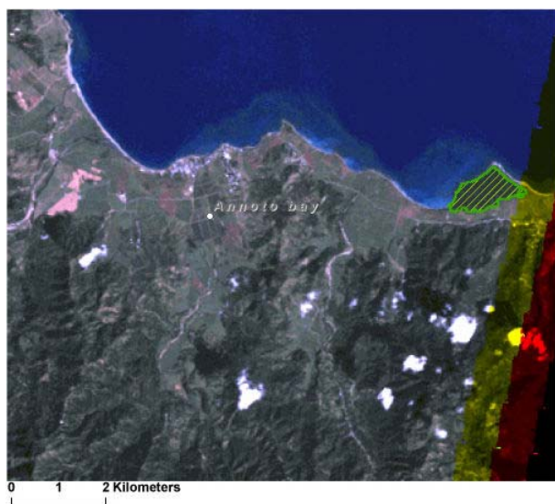
LS5 TM 29 January 1985
