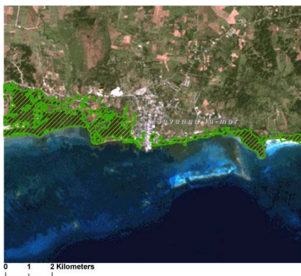
LS5 TM 17 February 1986
