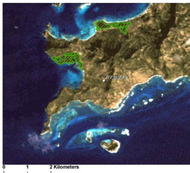
LS5 TM 19 January 1986
