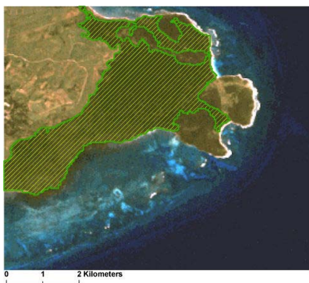
LS5 TM 9 January 1986 (Golden Grove)
