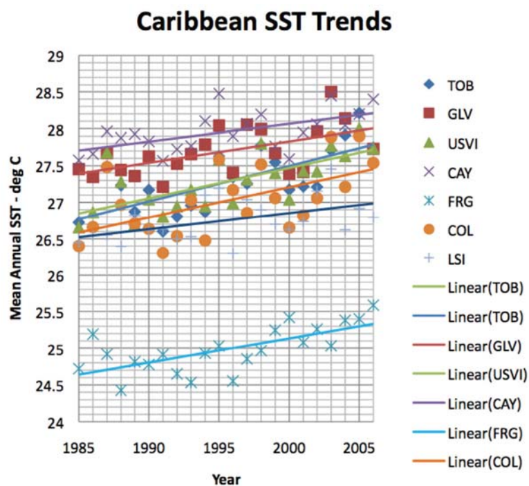
Figure 5 SST time series of seven representative Caribbean Virtual Stations (extracted from Simpson, et al. , 2009)
