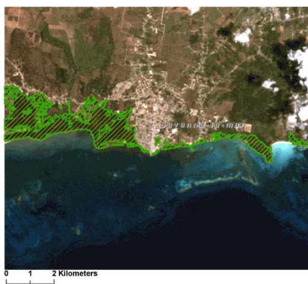
LS5 TM 11 April 2011
