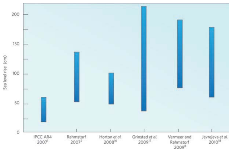
Figure 2 Ranges of sea level rise estimated for 2100 from semi-empirical models compared to IPCC AR4 (extracted from Rahmstorf 2010)
