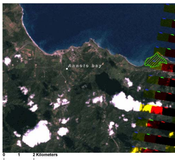
LS5 TM 18 January 2010
